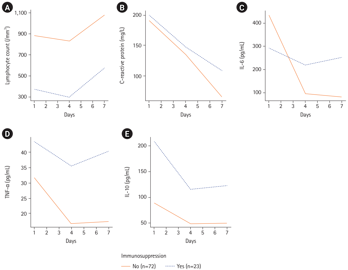
Supplementary Figure 4. Mean changes in (A) lymphocyte count, (B) C-reactive protein, (C) interleukin (IL)-6, (D) tumor necrosis factor (TNF)-α, and (E) IL-10 levels in immunocompetent and immunocompromised patients during the study period.
